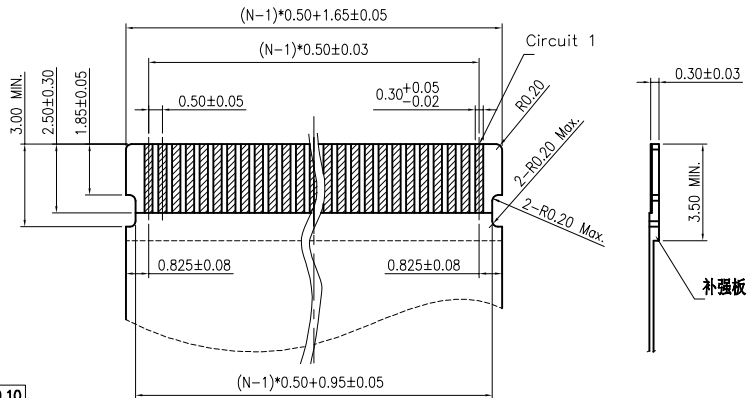
APPLICABLE FFC SPEC 公差:±0.05
